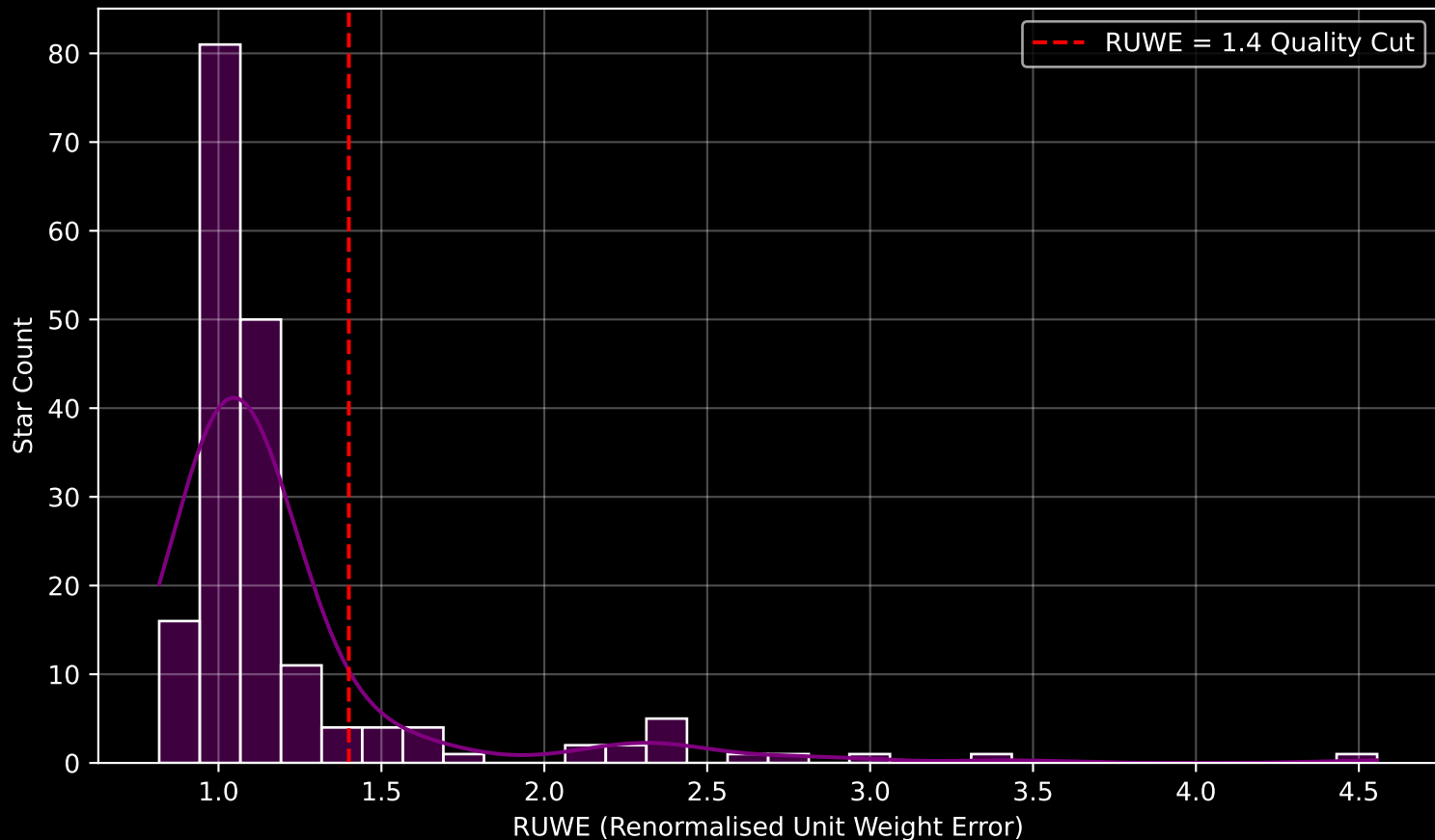
GAPOGEE DR17 Field [182+30_MGA] RUWE Distribution (n= 185)
