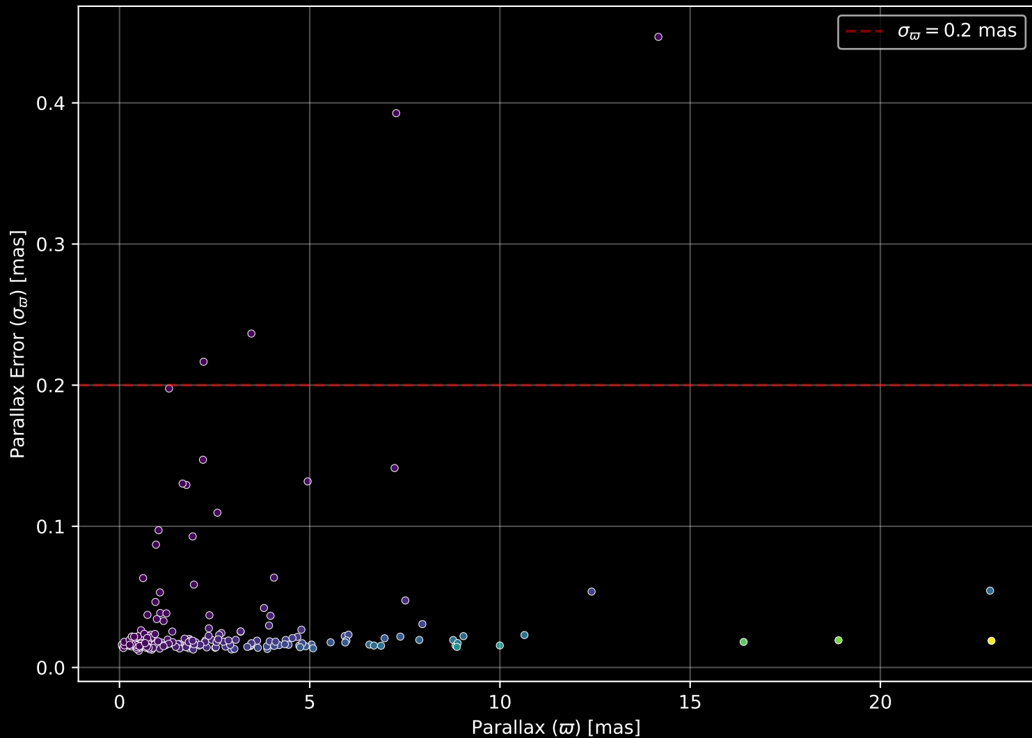
APOGEE DR17 Field: [182+30_MGA] Parallax Quality (n= 200)
