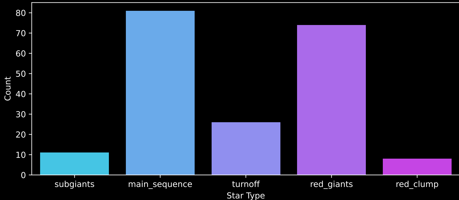
APOGEE DR17 Field: [182+30_MGA] Count plot of Star Type
