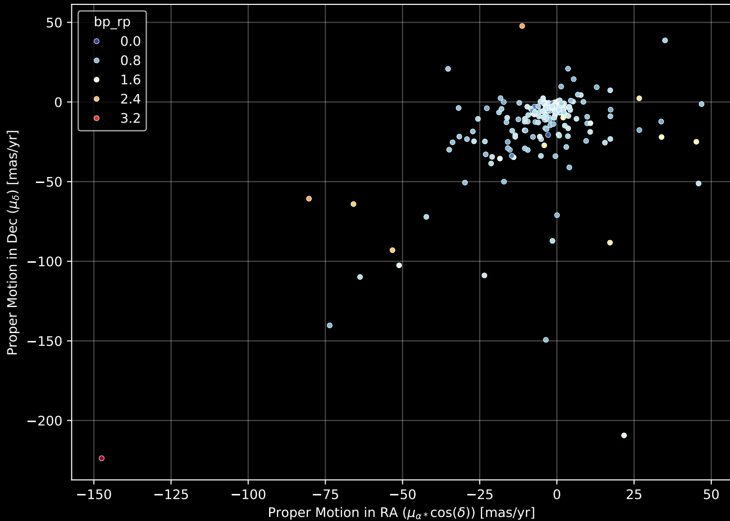
APOGEE DR17 Field: [182+30_MGA] Proper Motion Diagram (n= 200)
