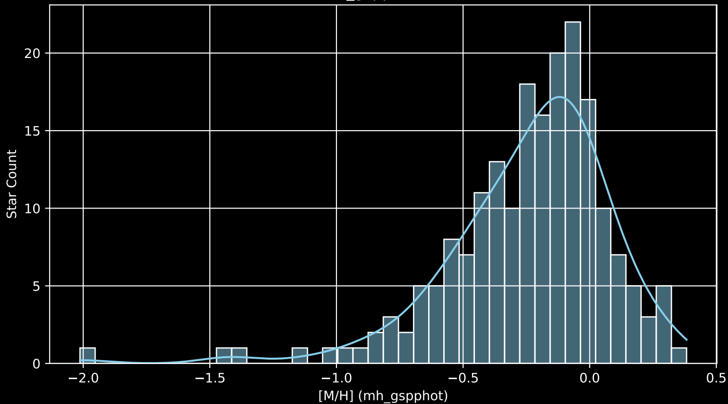
APOGEE DR17 Field: [182+30_MGA [M/H] (mh_gspphot) (n= 197)
